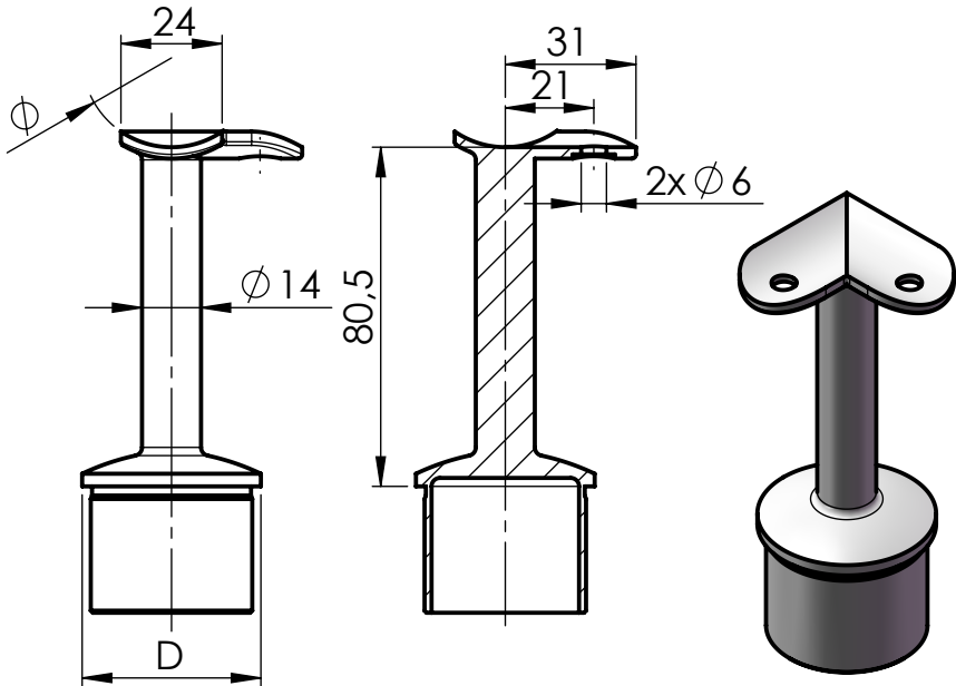
Saddle for flush angle A/0301-242
