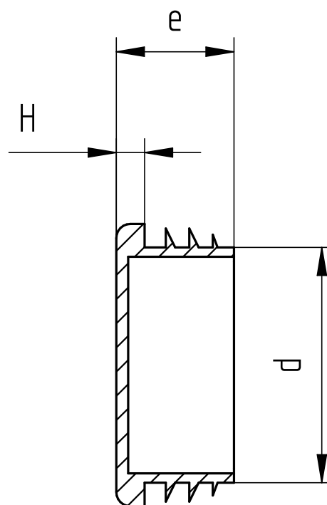
SECTION P-P
