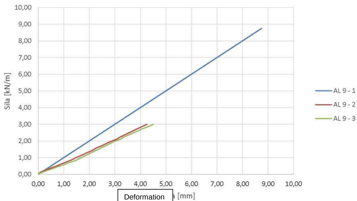
Graph of the dependence of the deformation of the lower edge of the profile on the force
