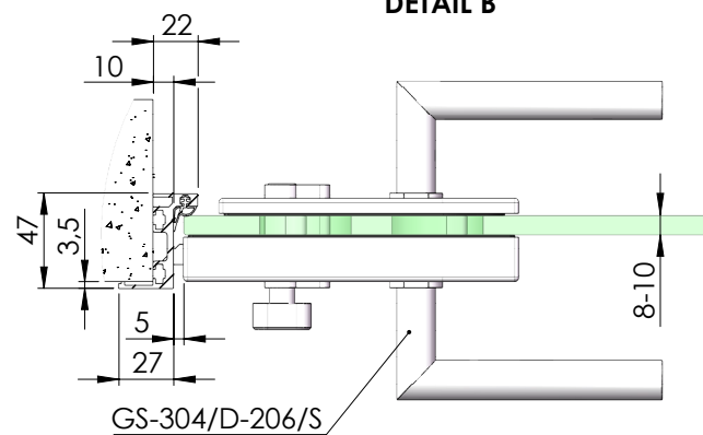
DETAIL B
