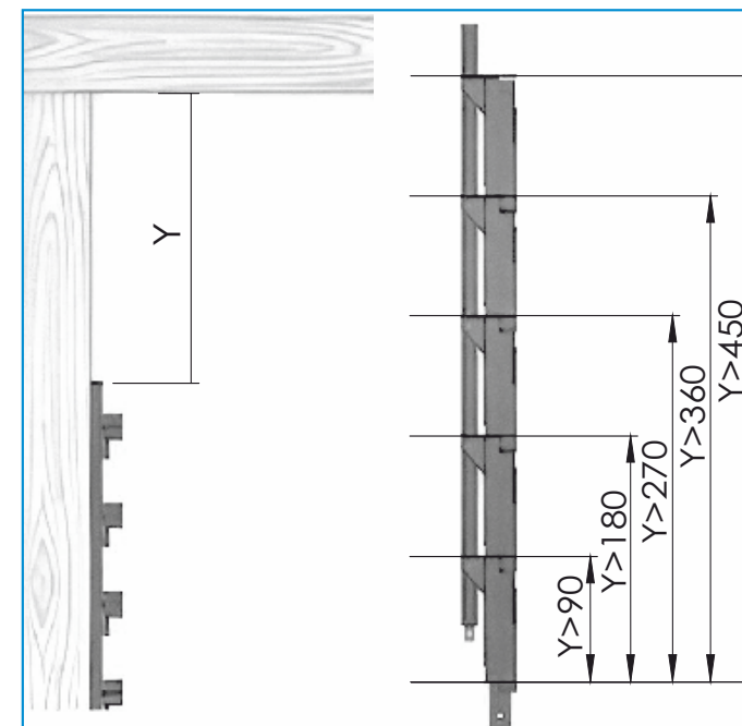
SEGMENT CUTTING - CUSTOM HEIGHTS
