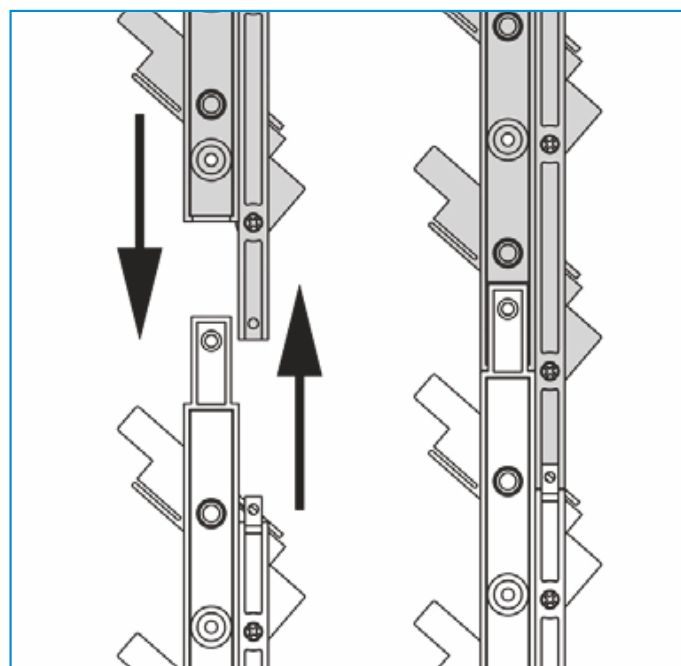
MODULAR SYSTEM - SEGMENTS STACKING
