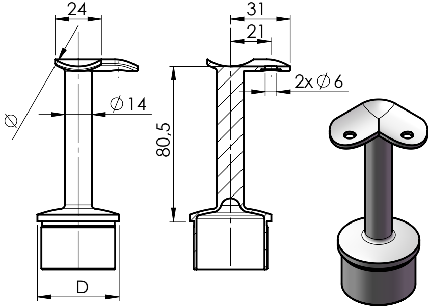
Saddle for flush angle A/0303-242
